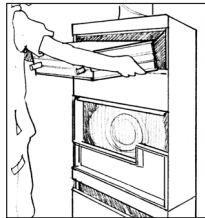
Fig. HWC-01 - Hot Water Coil easily slides into the fan coil
