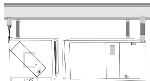
Fig. FCP-09 Attach Cooling Coil to Air Handler
