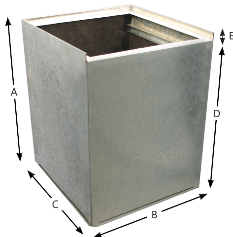
Fig. RA-03 – Hi-Velocity Return Air Base
