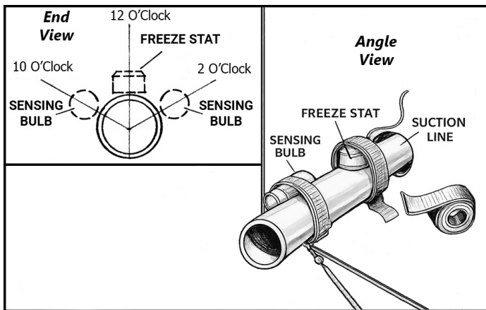
Fig. 15 - TX Sensing Bulb
