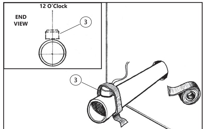
Fig. 03 - Anti-ice Control (Freeze Stat)
