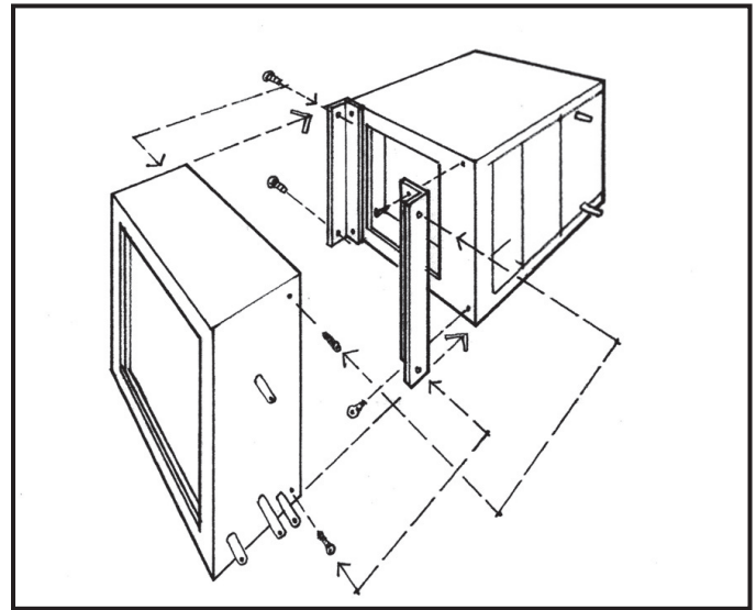
Fig. 02 - Mounting Brackets
